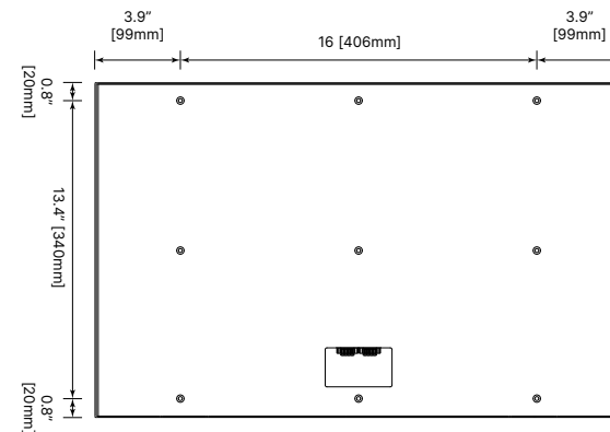
5 KEY LOCKER REAR ELEVATION w/ BACKPLATE NOT TO SCALE
