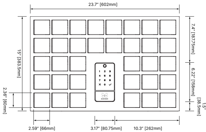
1 KEY LOCKER FRONT ELEVATION NOT TO SCALE
