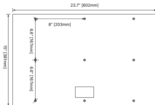
4 BACKPLATE FRONT ELEVATION NOT TO SCALE
