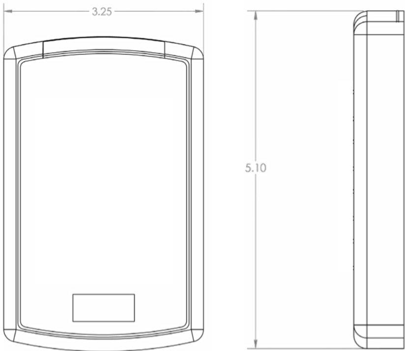
Front and Side Elevation
