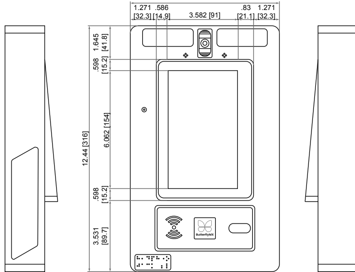
1 PANEL FRONT ELEVATION NOT TO SCALE
