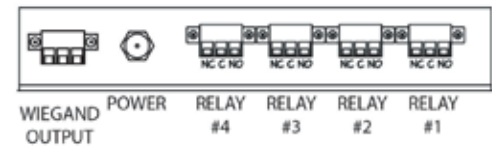
8 BOTTOM INTERFACE PANEL NOT TO SCALE
