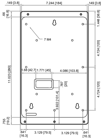
6 INTERCOM PANEL REAR w/ BACKPLATE NOT TO SCALE
