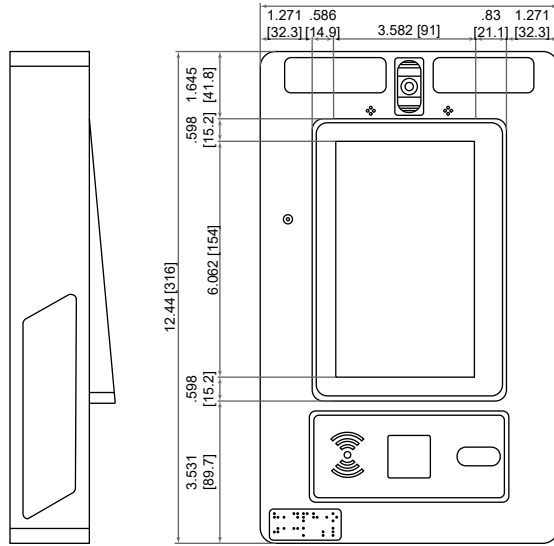
1 INTERCOM PANEL FRONT ELEVATION NOT TO SCALE
