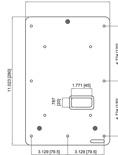
3 BACKPLATE FRONT ELEVATION
