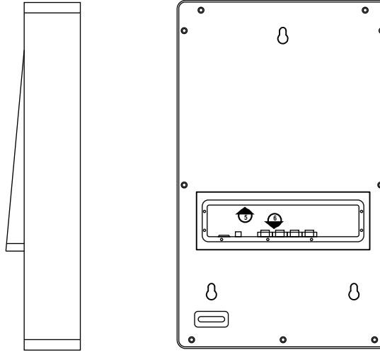
2 INTERCOM PANEL REAR ELEVATION NOT TO SCALE
