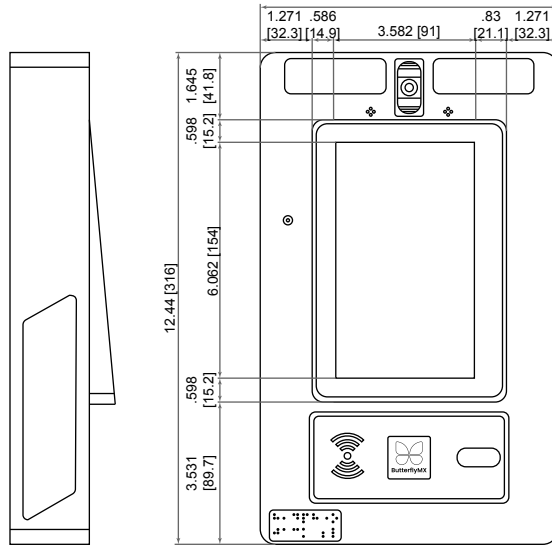
1 INTERCOM FRONT ELEVATION
