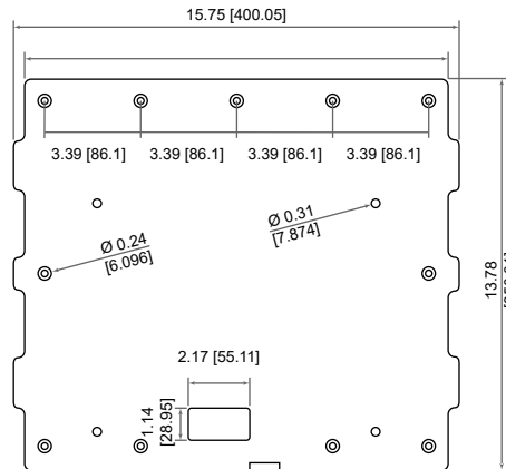
5 BACKPLATE FRONT ELEVATION NOT TO SCALE
