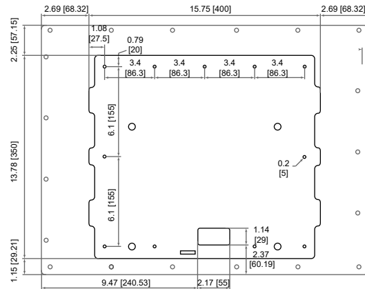
4 INTERCOM REAR ELEVATION w/ BACKPLATE NOT TO SCALE
