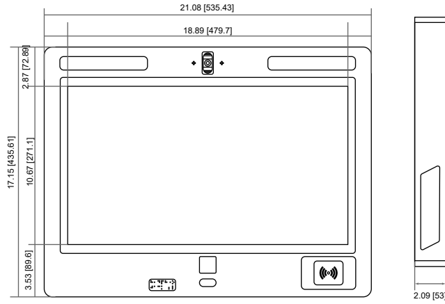
1 INTERCOM PANEL FRONT ELEVATION NOT TO SCALE
