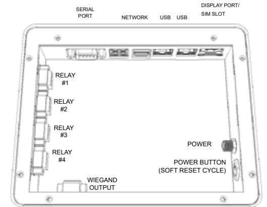
6 I/O PORT VIEW NOT TO SCALE
