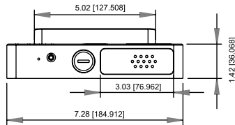
4 INTERCOM BOTTOM ELEVATION NOT TO SCALE
