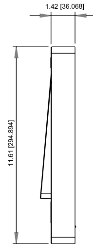
3 INTERCOM SIDE ELEVATION NOT TO SCALE
