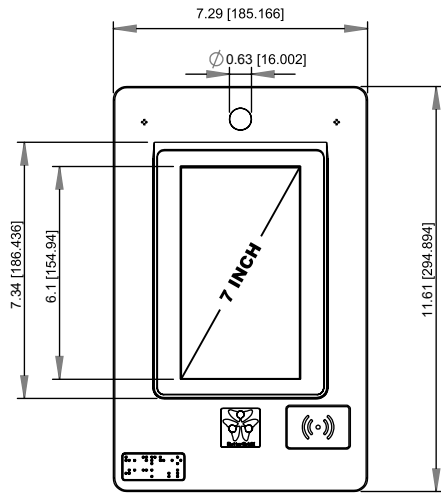
1 INTERCOM FRONT ELEVATION NOT TO SCALE
