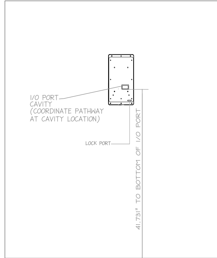
2 REAR VIEW: BACKPLATE PLACEMENT NOT TO SCALE
