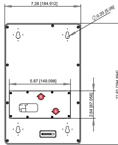
2 INTERCOM BACK ELEVATION NOT TO SCALE
