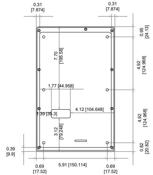
8 INTERCOM REAR ELEVATION w/ BACKPLATE NOT TO SCALE
