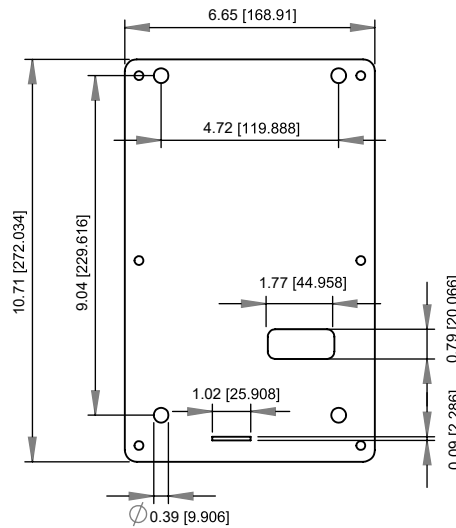
7 BACKPLATE FRONT ELEVATION NOT TO SCALE
