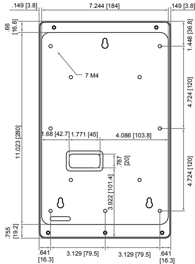
6 INTERCOM REAR w/ BACKPLATE NOT TO SCALE
