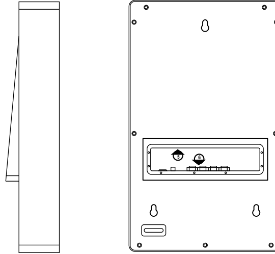
2 INTERCOM REAR ELEVATION NOT TO SCALE
