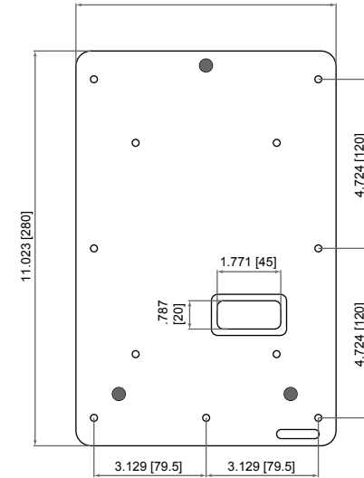
3 BACKPLATE FRONT ELEVATION NOT TO SCALE
