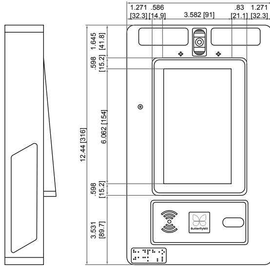
1 INTERCOM FRONT ELEVATION NOT TO SCALE
